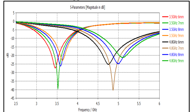
Fig.7. Effect of The Width of The Shorting Plate
