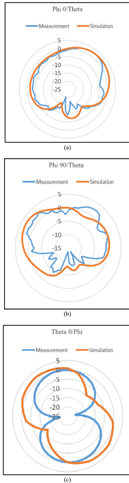
Fig. 9. Simulated & Measured Radiation Pattern at 4.8GHz Frequency (a) XZ plane (b) YZ plane (c) XY plane
