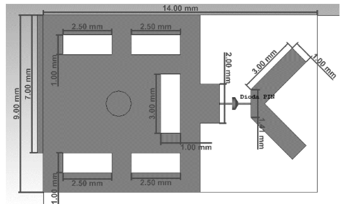
Fig. 2. Top View of Radiating Patch
