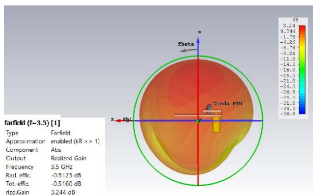
Fig. 10. Simulated Radiation Pattern in 3D at 3.5GHz
