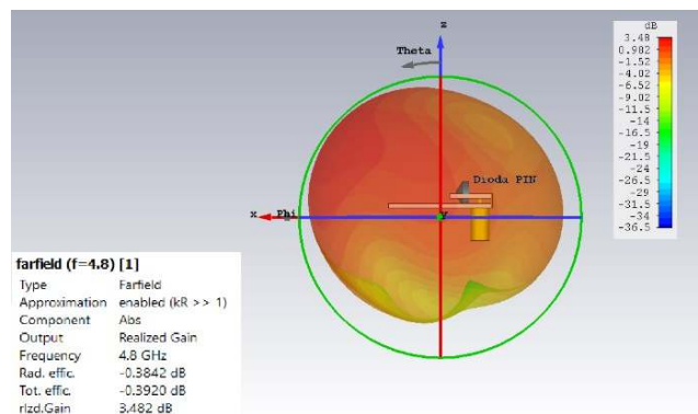
Fig. 11. Simulated Radiation Pattern in 3D at 4.8GHz
