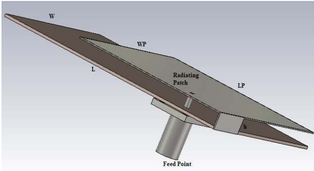
Fig. 1. Structure of PIFA Antenna
