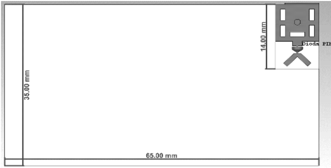
Fig. 3. Top View of Whole Structure
