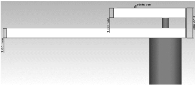
Fig. 4. Side View of Whole Structure
